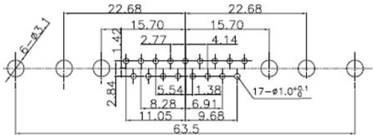
PCB Layout
